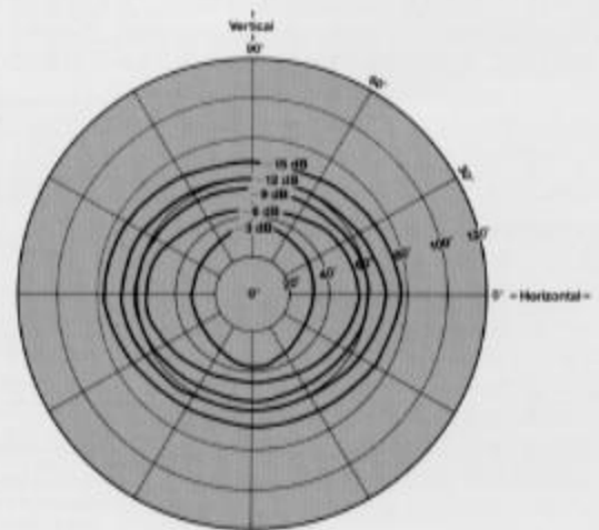
8 kHz octave bandwidth constant sound pressure contours. Same conditions as 1 kHz contours.
