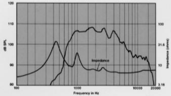
Frequency response of the 2344A, measured on axis at a distance of 1 meter with 1 watt (2.24 V rms) applied to a JBL Model 2426H compression driver (impedance minimum 5 ohms), in a reflection free environment, with impedance vs. frequency curve.
