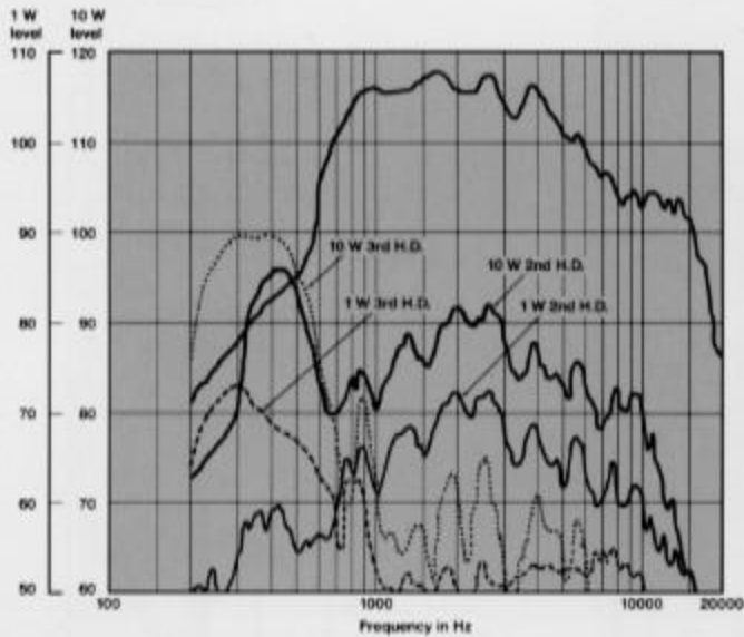
Second and third harmonic distortion curves of the 2344A with 1 watt (2.24 V rms) and 10 watts (7.1 V rms) applied to the JBL Model 2426H compression driver (impedance minimum 5 ohms). Measured on axis at a distance of 1 meter in a reflection free environment.
