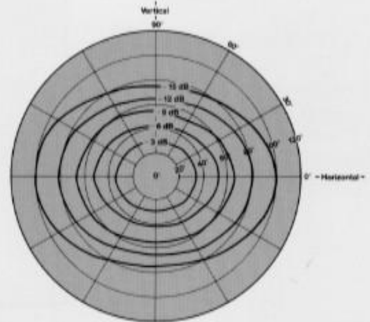
2 kHz octave bandwidth sound pressure contours. Same conditions as 1 kHz contours.
