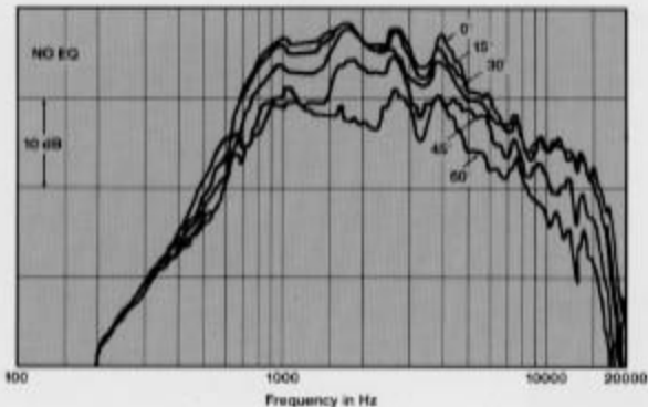
Horizontal off-axis response taken at 15° intervals out to 60° off axis. Both normalized (equalized flat on axis) and unequalized response are shown.
