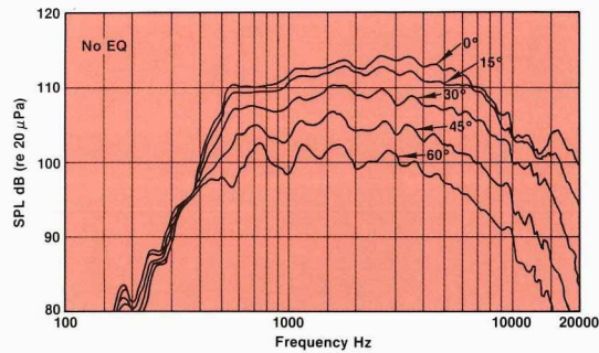
Horizontal off-axis response. Horizontal off-axis response taken at 15 degree intervals out to 60° off axis. Both normalized (equalized flat on axis) and unequaled responses are shown.
