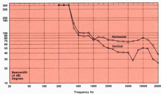
Directivity vs Frequency
