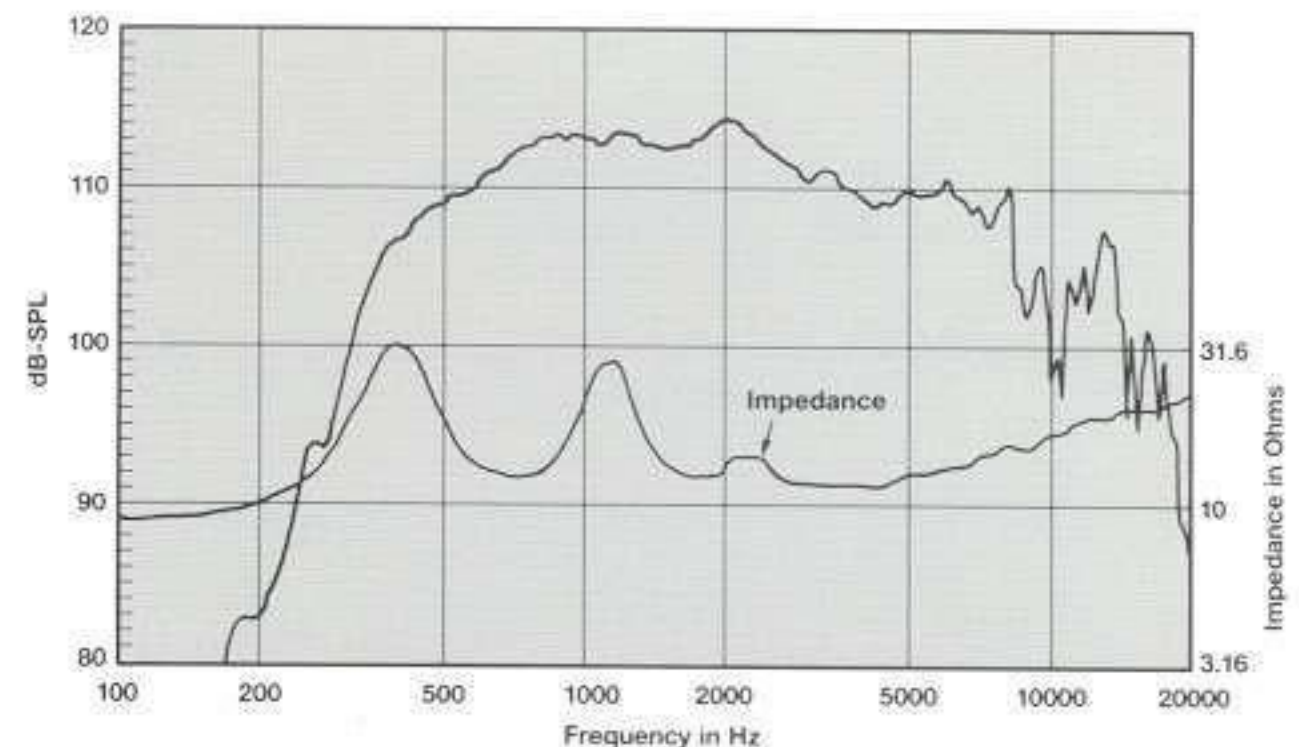
Response on JBL 2352 Bi-Radial® Horn
