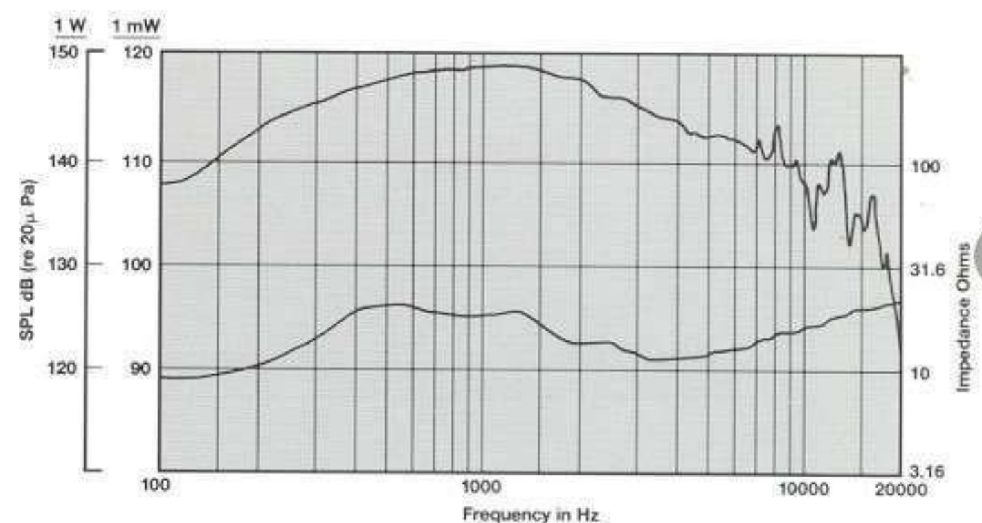
Response on Plane-Wave Terminated Tube
