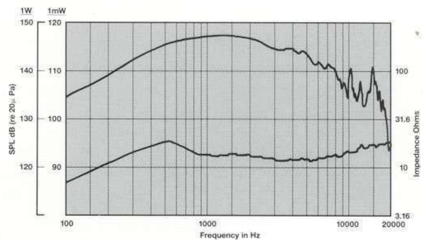
Response on Plane-Wave Terminated Tube
