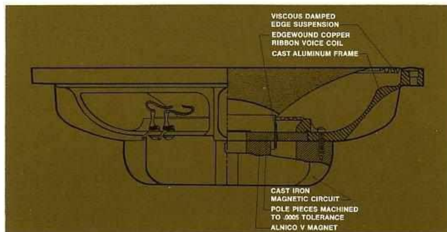
Section drawing of 12-inch low frequency transducer.
