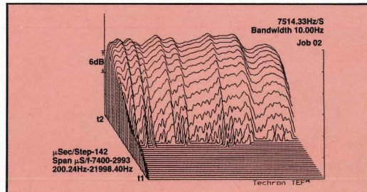
Time-Energy-Frequency (TEF) Curves (200 Hz to 22 kHz) Front-back span is from 7400 microseconds to 2993 microseconds; vertical divisions 6 dB. Note the smooth decay of the system and high frequency extension beyond 20 kHz.
