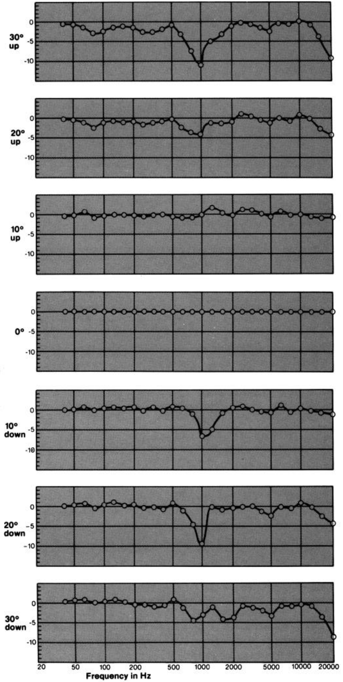
Figure 5. Vertical Off-axis Response (normalize to on-axis)
