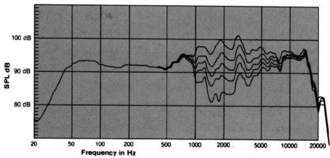
Figure 7. Control Range, Mid (4430)
