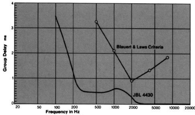
Figure 6. Group Delay vs. Blauert & Laws Criteria
