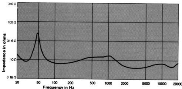
Figure 9. Impedance (4430)
