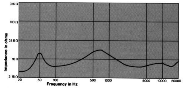
Figure 10. Impedance (4435)
