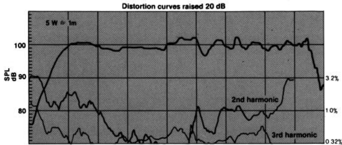
Figure 15. Distortion vs. Frequency (4430)
