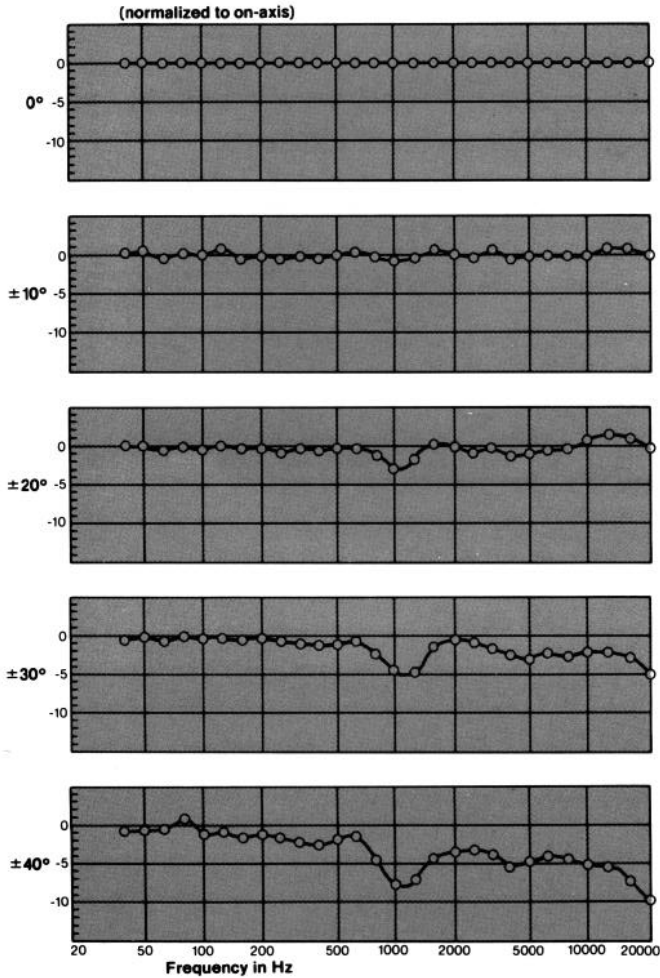
Figure 4. Horizontal Off-axis Response
