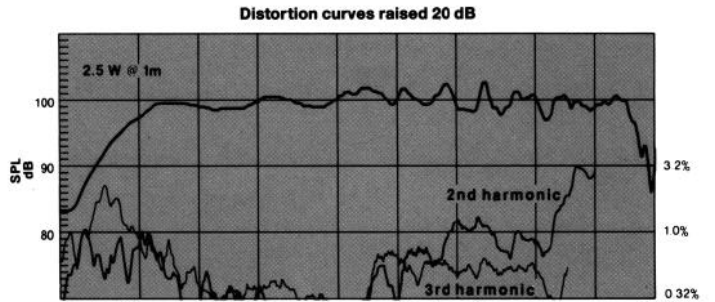
Figure 16. Distortion vs. Frequency (4435)
