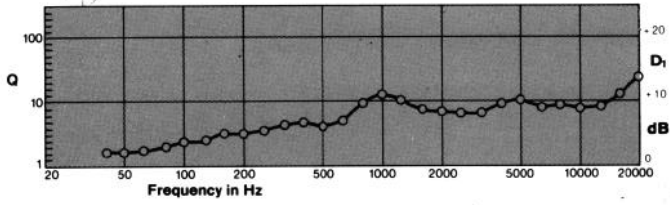
Figure 3. Directivity vs. Frequency (4430)
