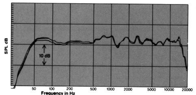
Figure 13. Power Linearity (4430), 1 W, 10 W, 100 W @ 1 m: (Average Axial Level of 93 dB, 103 dB, 113 dB SPL)
