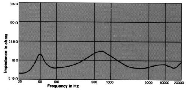
Figure 10. Impedance (4435)
