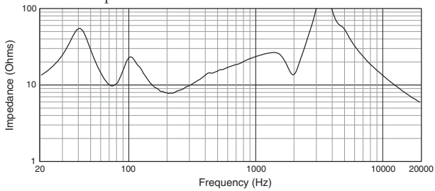
Horizontal Impedance
