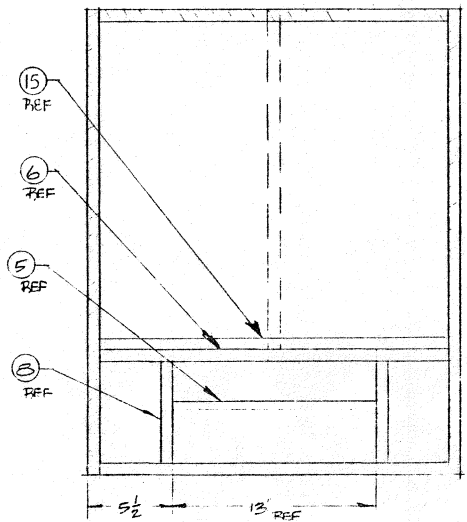
SECT B-B
