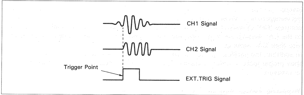
Figure 6. EXT.TRIG
