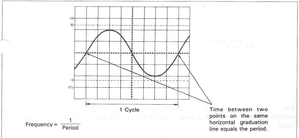
Figure 12. Measuring Frequency
