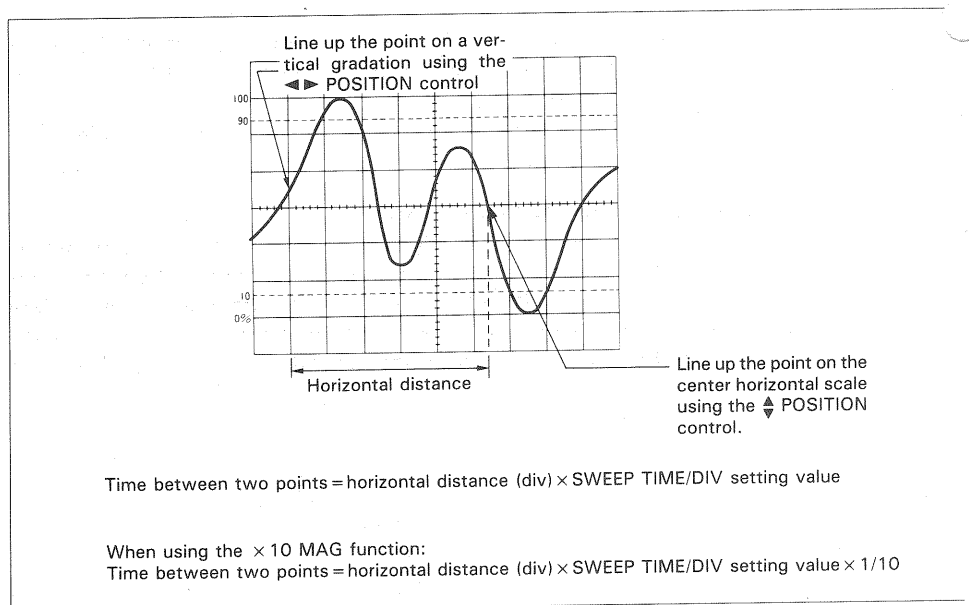
Figure 11. Time Measurement
