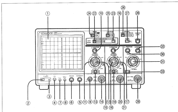
Figure 1. Front Panel
