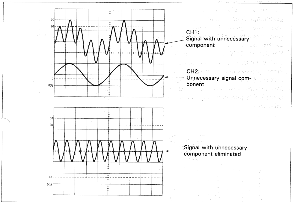
Figure 8. Common-Mode Rejection
