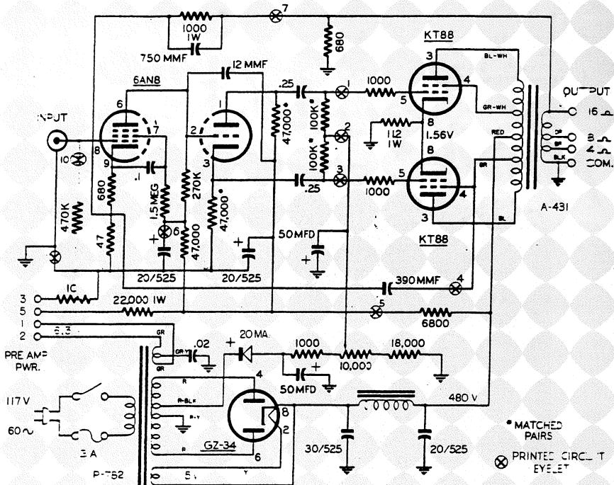
DYNAKIT MARK III 60 WATT POWER AMPLIFIER
