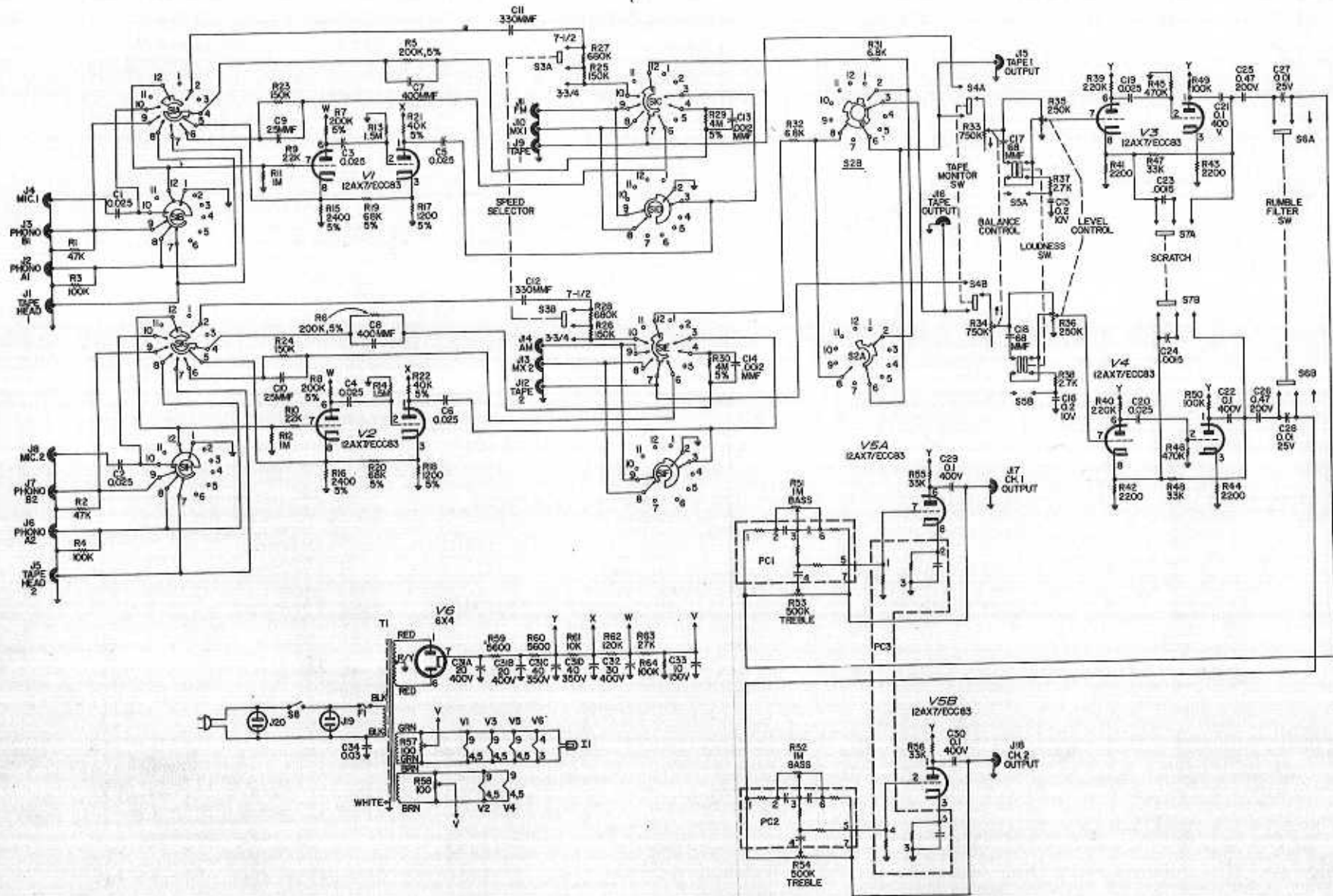
Figure 5-6. ST-84 Schematic Diagram
