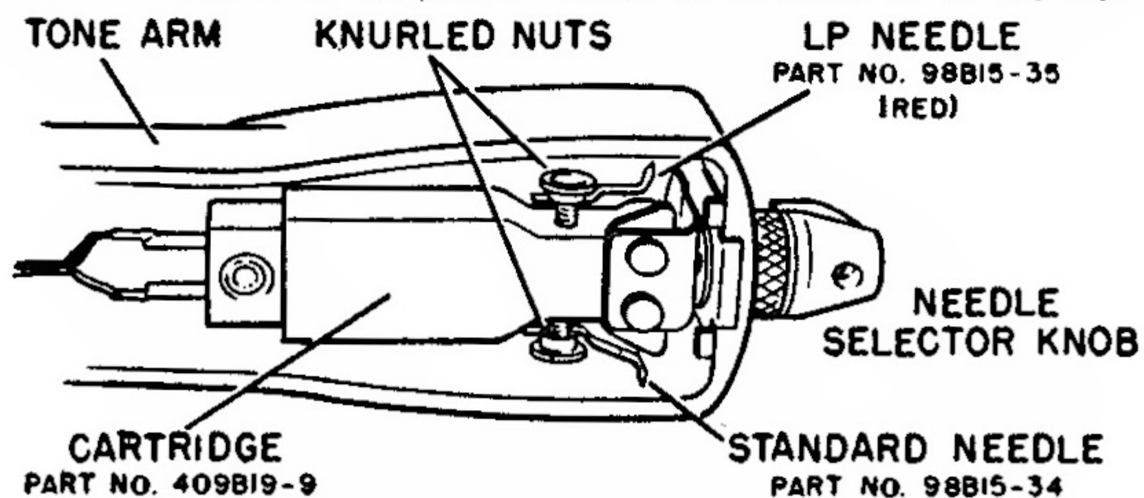
Bottom View of Cartridge and Needles.
