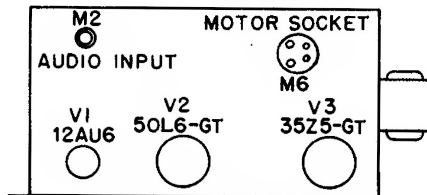
Side View of Chassis.
