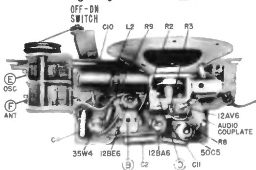
Top View of Chassis. Location of Components and Alignment Adjustments Shown.
