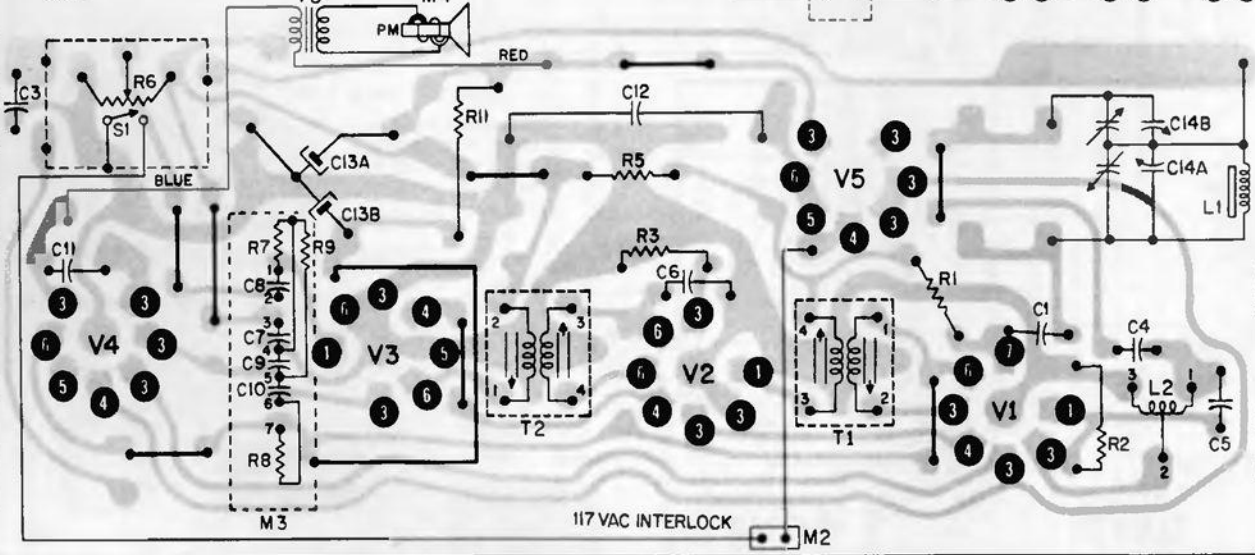
Bottom View of Etched Circuit Board. Gray area represents etched wiring; black symbols and lines represents components and connections on opposite side.
