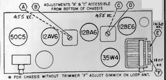
Top View of Chassis Showing Tube and Alignment Points Locations.
