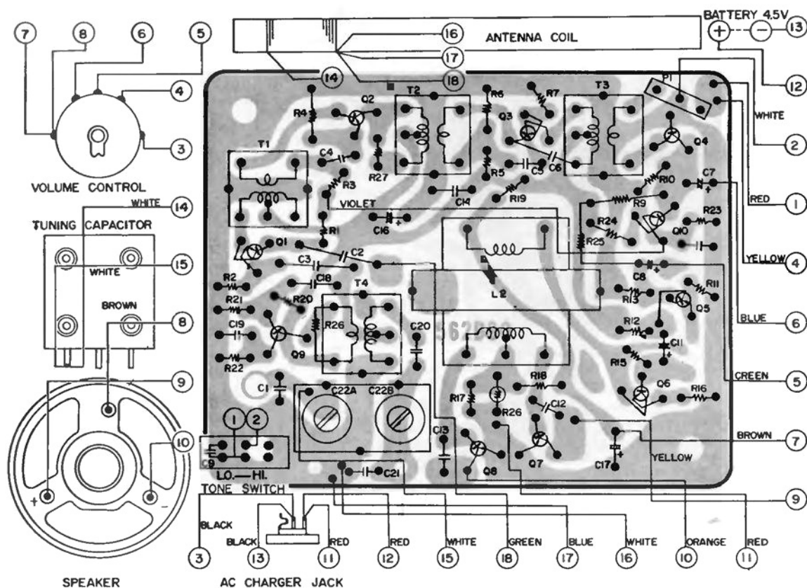
COMPONENT CONNECTIONS TO BACK OF BOARD & WIRING
