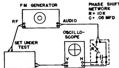
FIG. 2 INSTRUMENT CONNECTIONS
