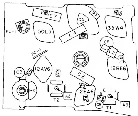
LOCATION OF PARTS UNDER CHASSIS
