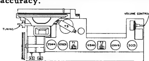
TUBE LAYOUT
