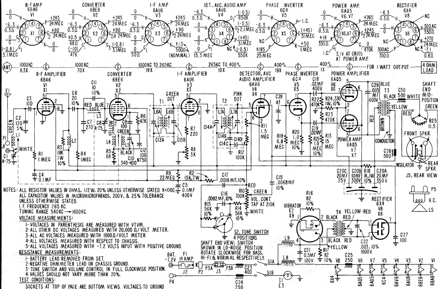
BENDIX RADIO Serial Nos. 5BH and 5BM, Models R5BLA, R5BLB, R5BM, used in Lincoln-Mercury, No. FDL-18805-B, -C, -D
