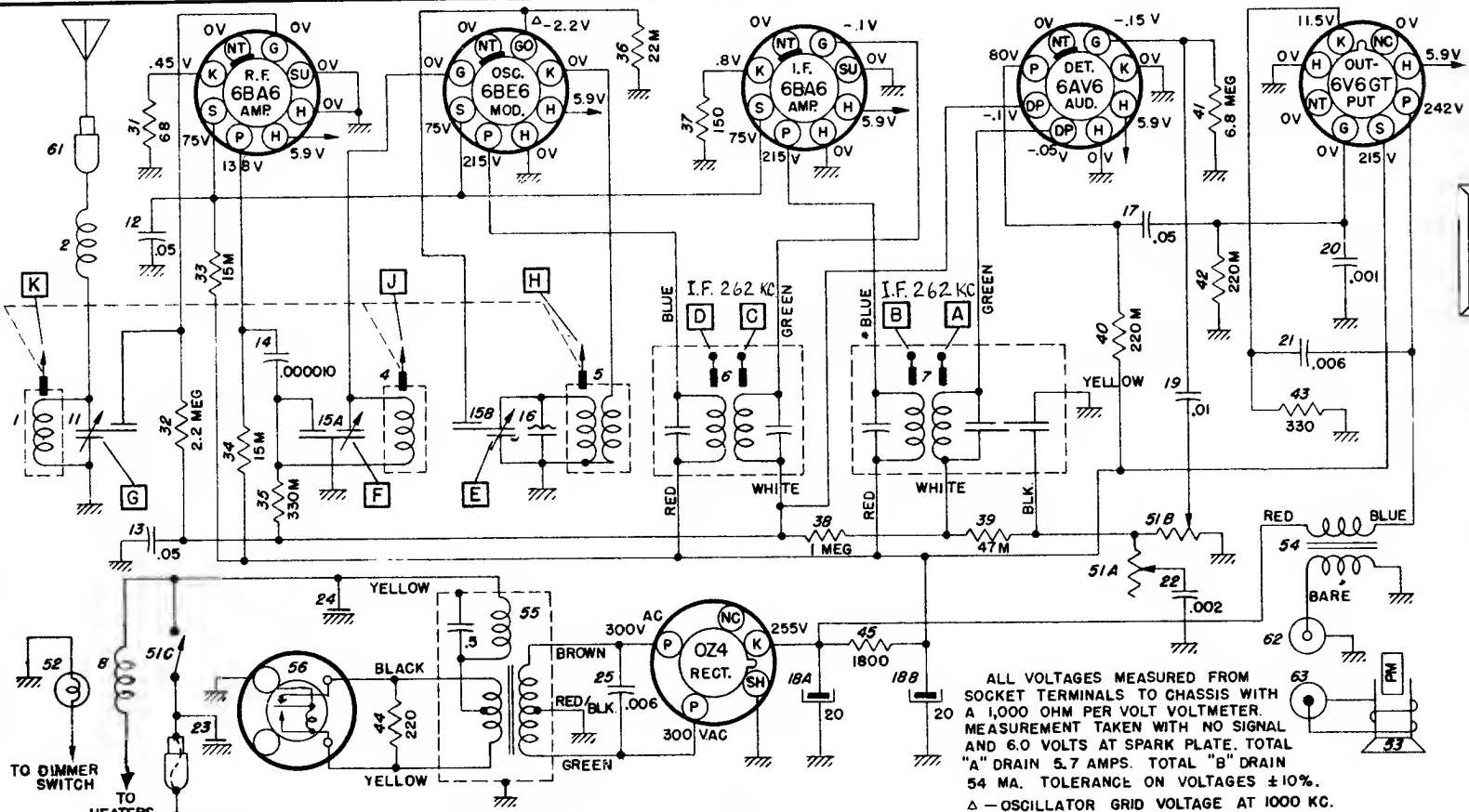
CIRCUIT DIAGRAM—986669
