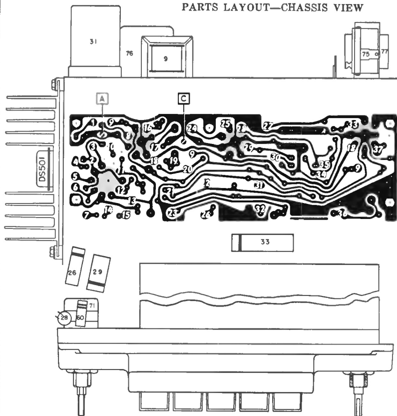
PARTS LAYOUT—CHASSIS VIEW
