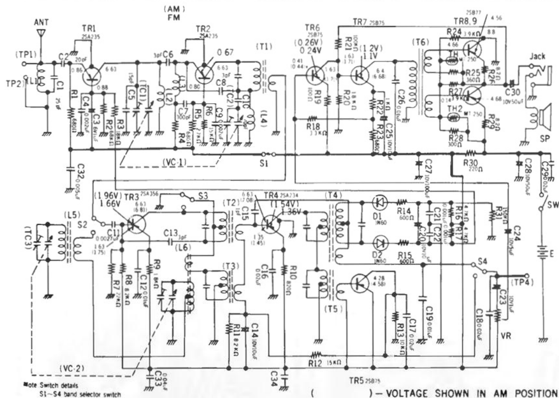
VOLTAGE AND CURRENT AT ELEMENT OF TRANSISTOR
