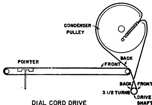
DIAL CORD DRIVE
