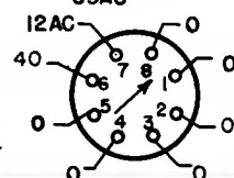
Socket Voltage Diagram
