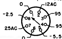
Socket Voltage Diagram
