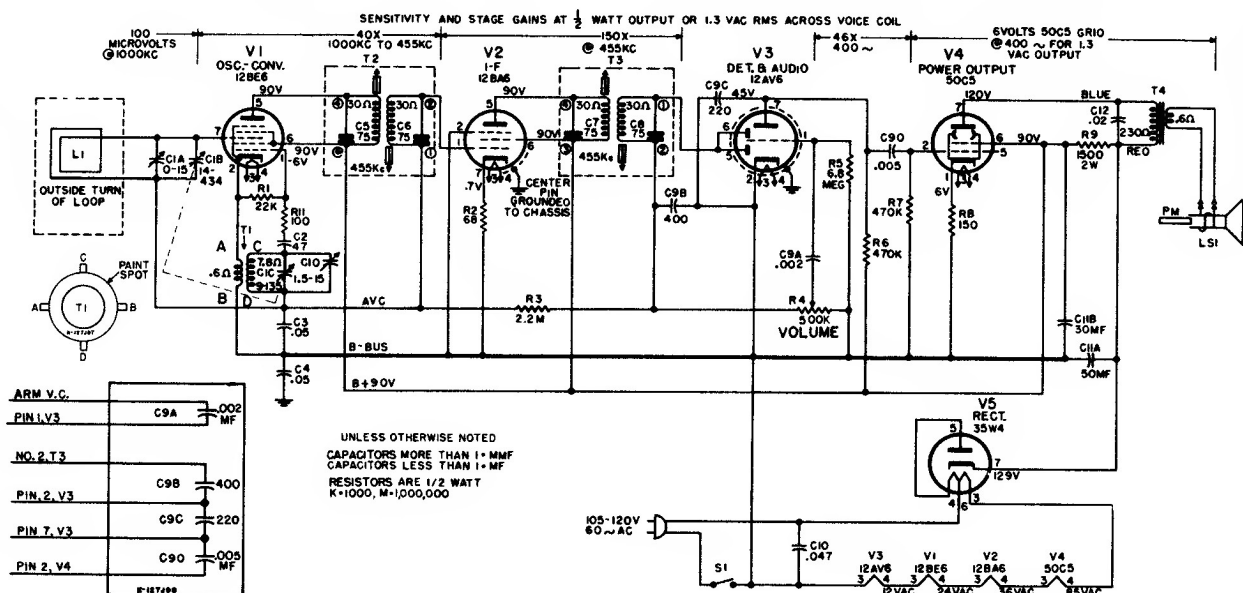
ALIGNMENT CHART
