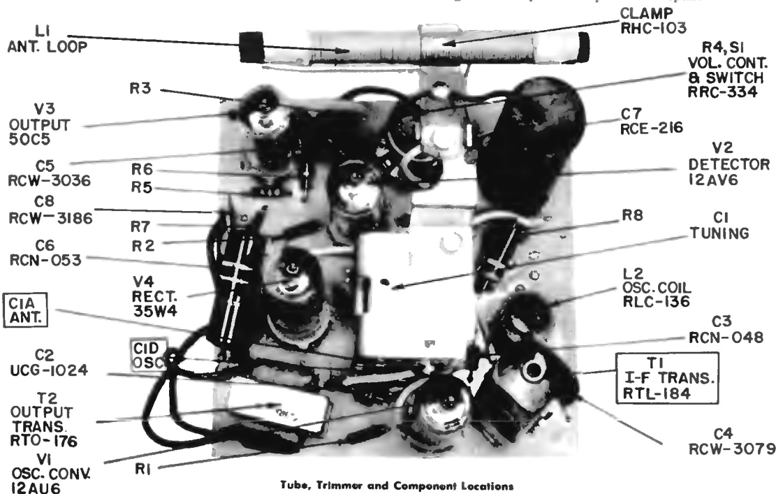
Tube, Trimmer and Component Locations
