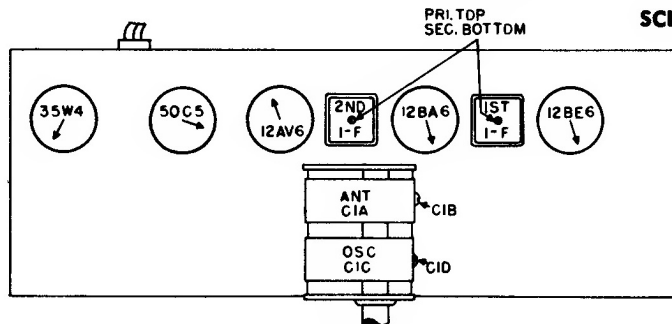
TUBE AND TRIMMER LOCATION
