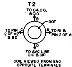
Osc. Coil Wiring
