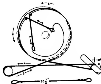
Dial Cord Stringing
