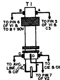
R-F Coil Wiring
