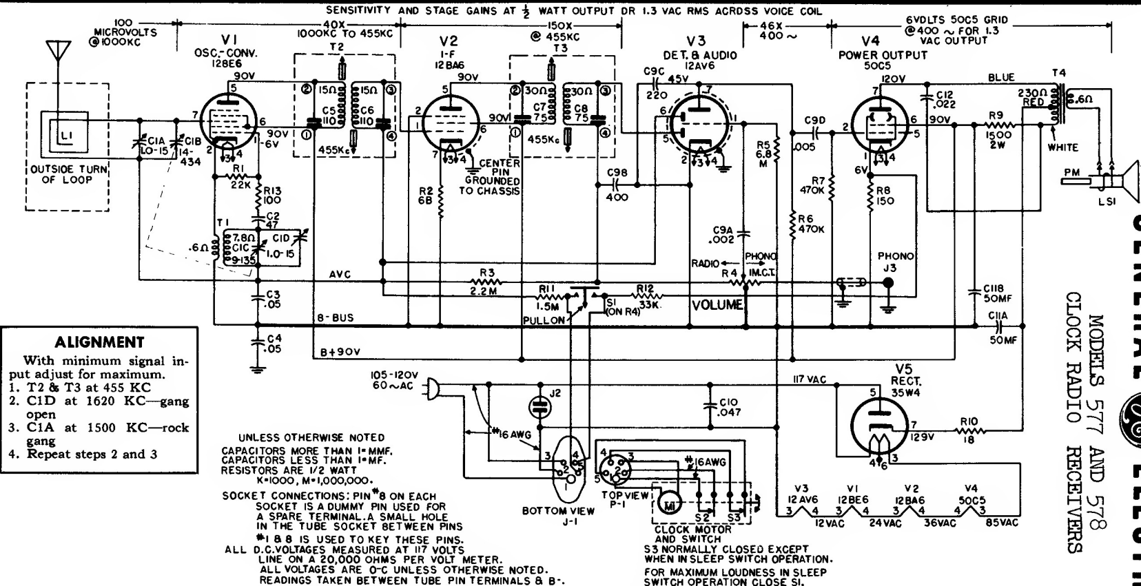
Schematic Diagram, Models 577 and 578
