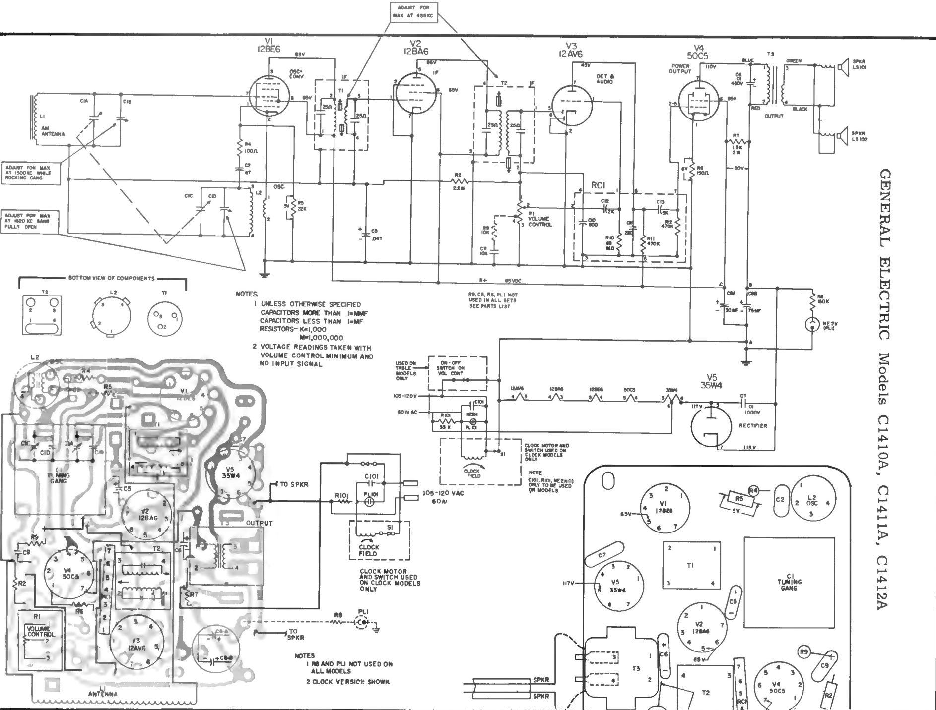
COMPONENT WIRING DIAGRAM (BOTTOM VIEW) RADIO MODEL C1410
