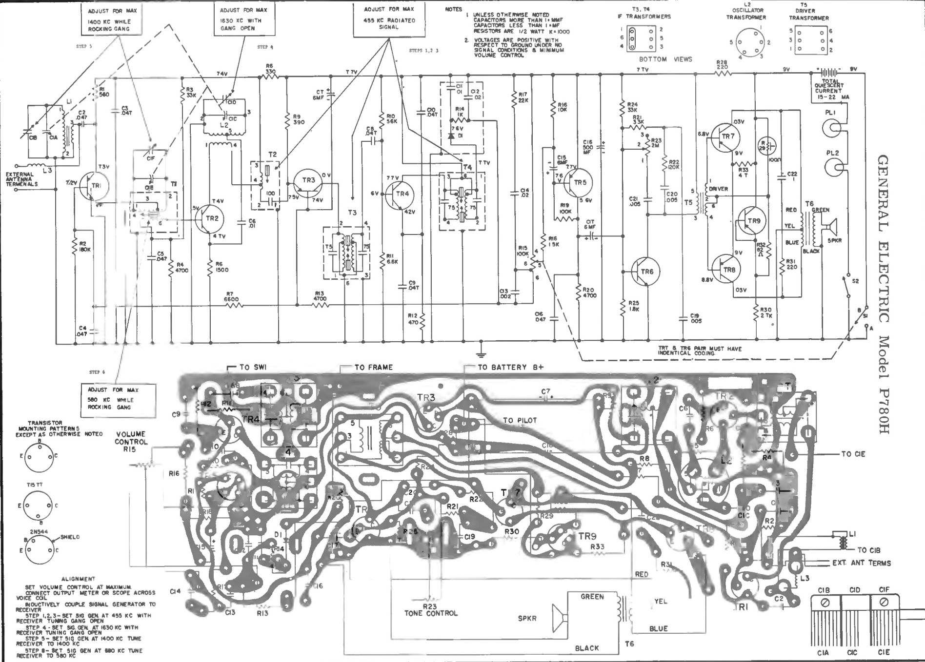
MODEL P780H WIRING DIAGRAM - BOTTOM VIEW
