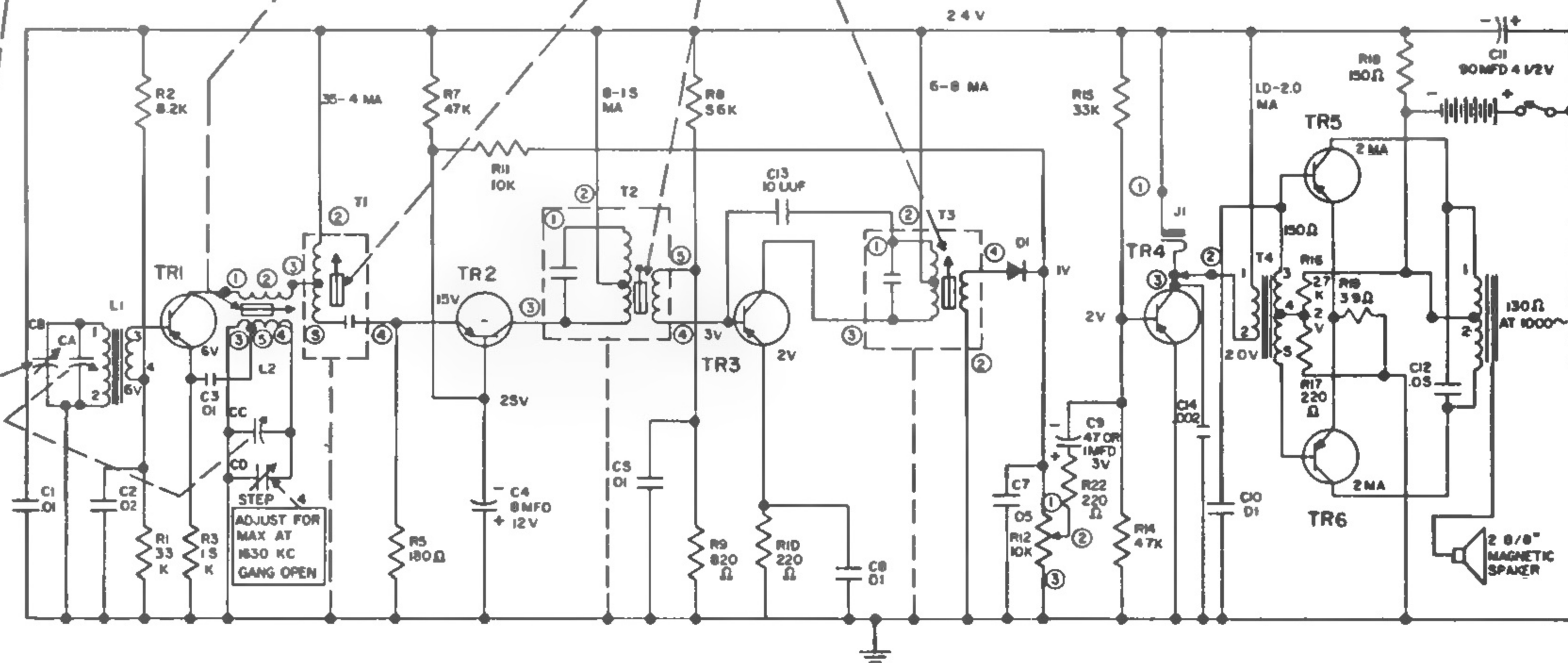
COMPONENT WIRING DIAGRAM
