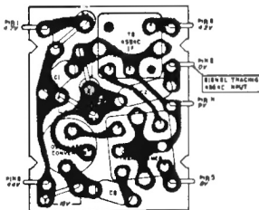
TOP VIEW CONVERTER (CM-3)
