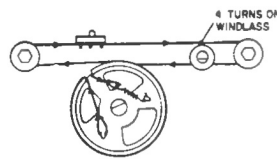
STRINGING DIAGRAM
