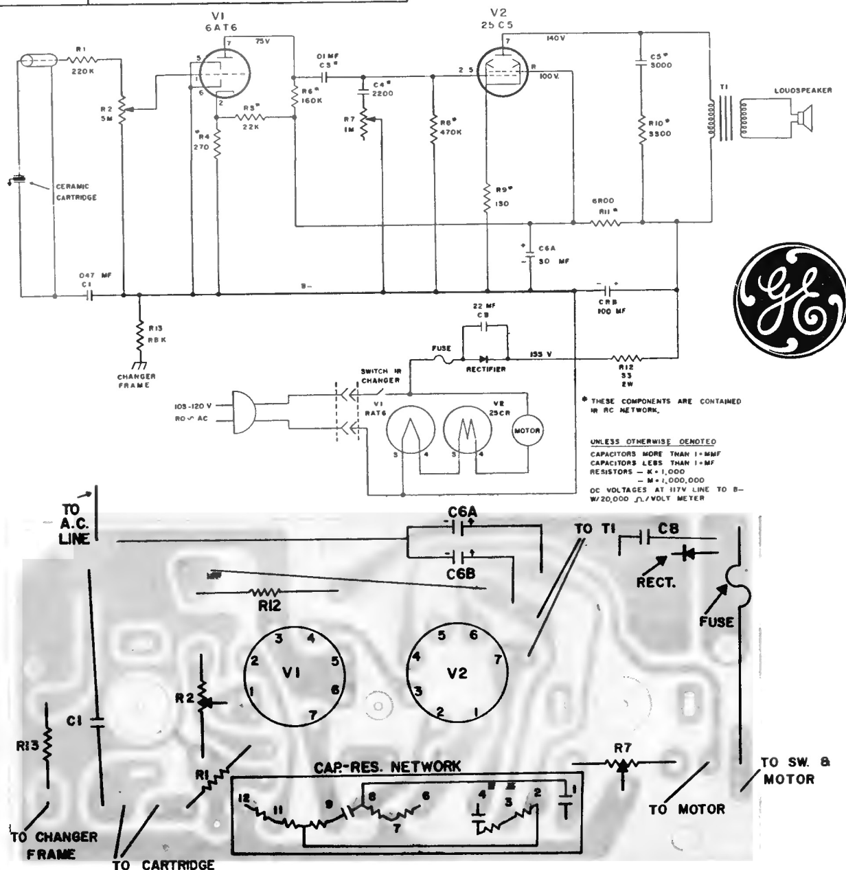
COMPONENT LOCATIONS - BOTTOM VIEW - RP-III0A
