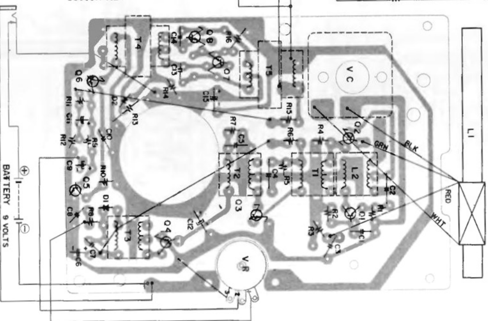
CIRCUIT BOARD LAYOUT (VIEWED FROM COPPER SIDE)
