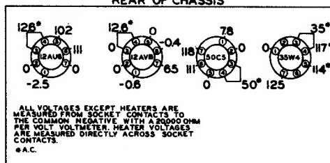
VOLTAGE TABLE (BOTTOM VIEW OF CHASSIS)
