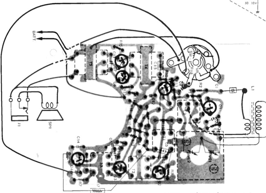
Bottom View of PC Board.
