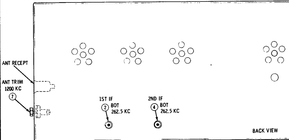
ALIGNMENT POINTS LOCATION DETAIL
