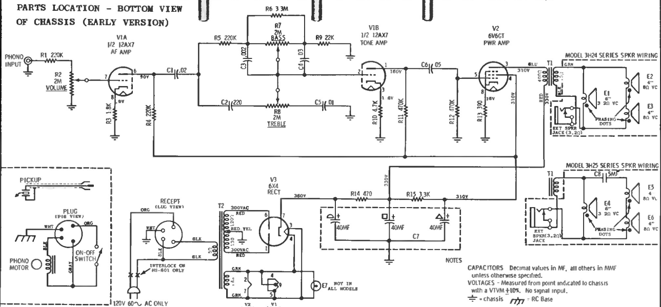
SCHEMATIC DIAGRAM (EARLY VERSION)
