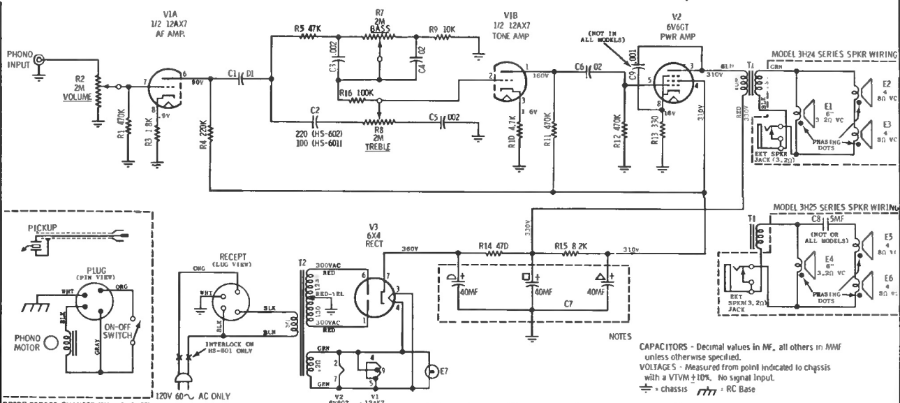
SCHEMATIC DIAGRAM (LATE VERSION)
