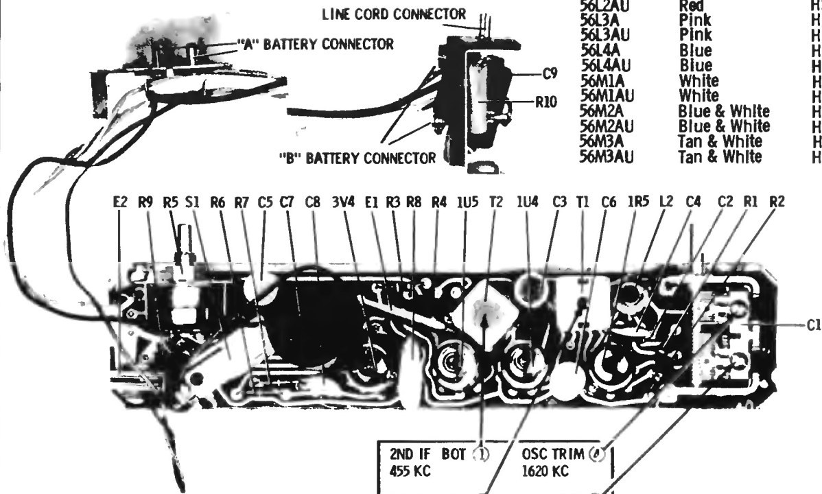
ALIGNMENT ADJUSTMENTS AND PARTS LOCATION
