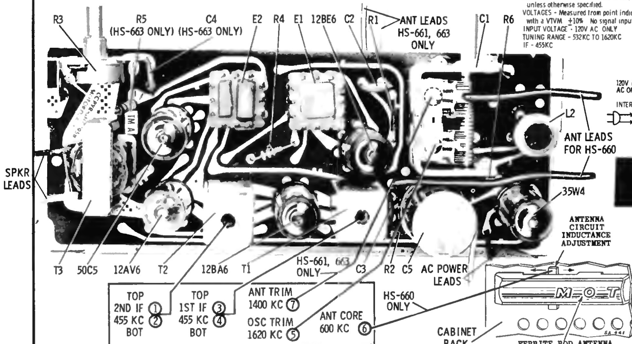
HS-660, 661 & 663 ALIGNMENT POINTS & PARTS LOCATIONS
