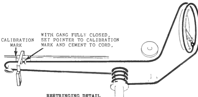
RESTRINGING DETAIL
