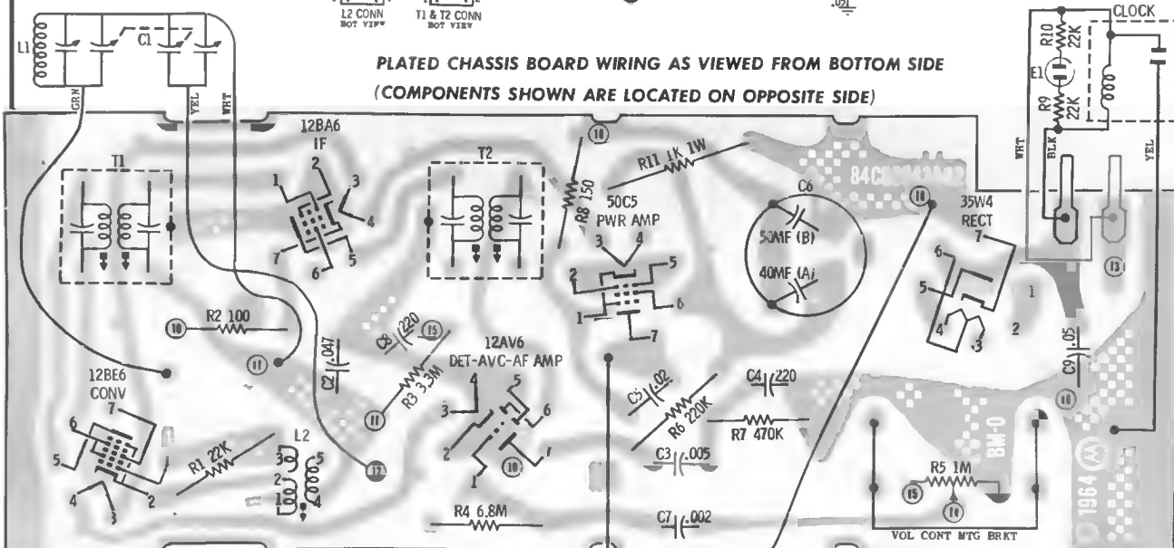
BOTTOM VIEW
