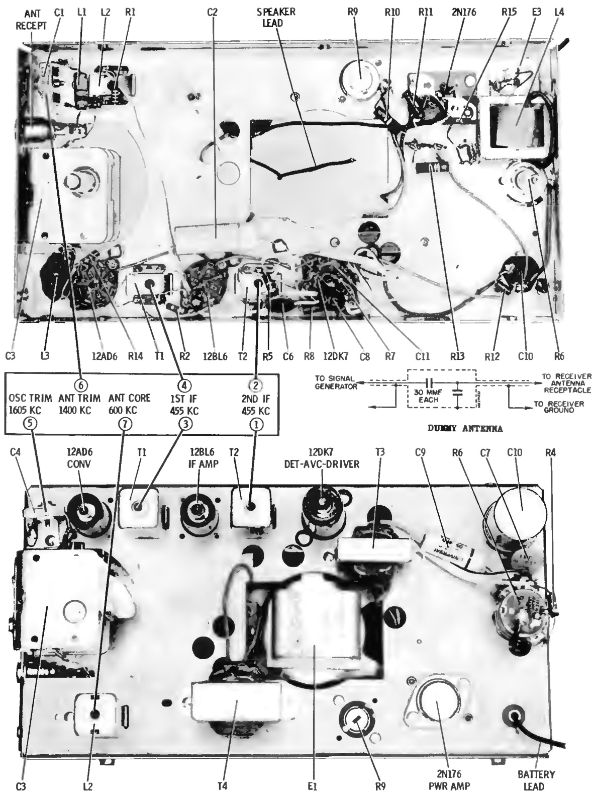
ALIGNMENT ADJUSTMENTS AND PARTS LOCATIONS
