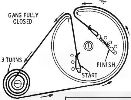
DIAL STRINGING DETAIL
