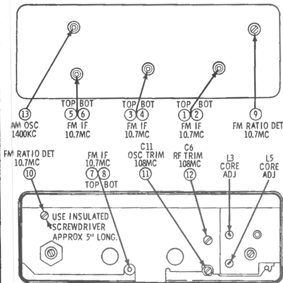
FMC62 ALIGNMENT LOCATION POINTS
