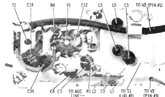
MODEL FMC62 TUNER PARTS LOCATION
