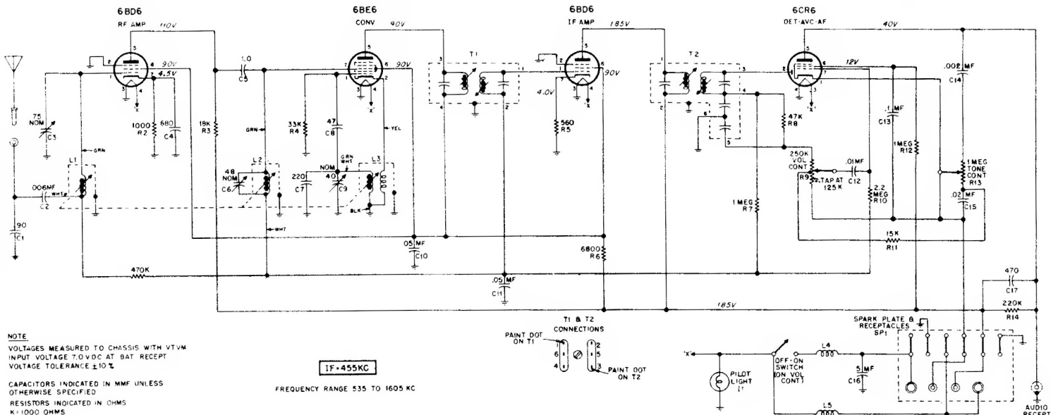
R17A6 SCHEMATIC DIAGRAM
