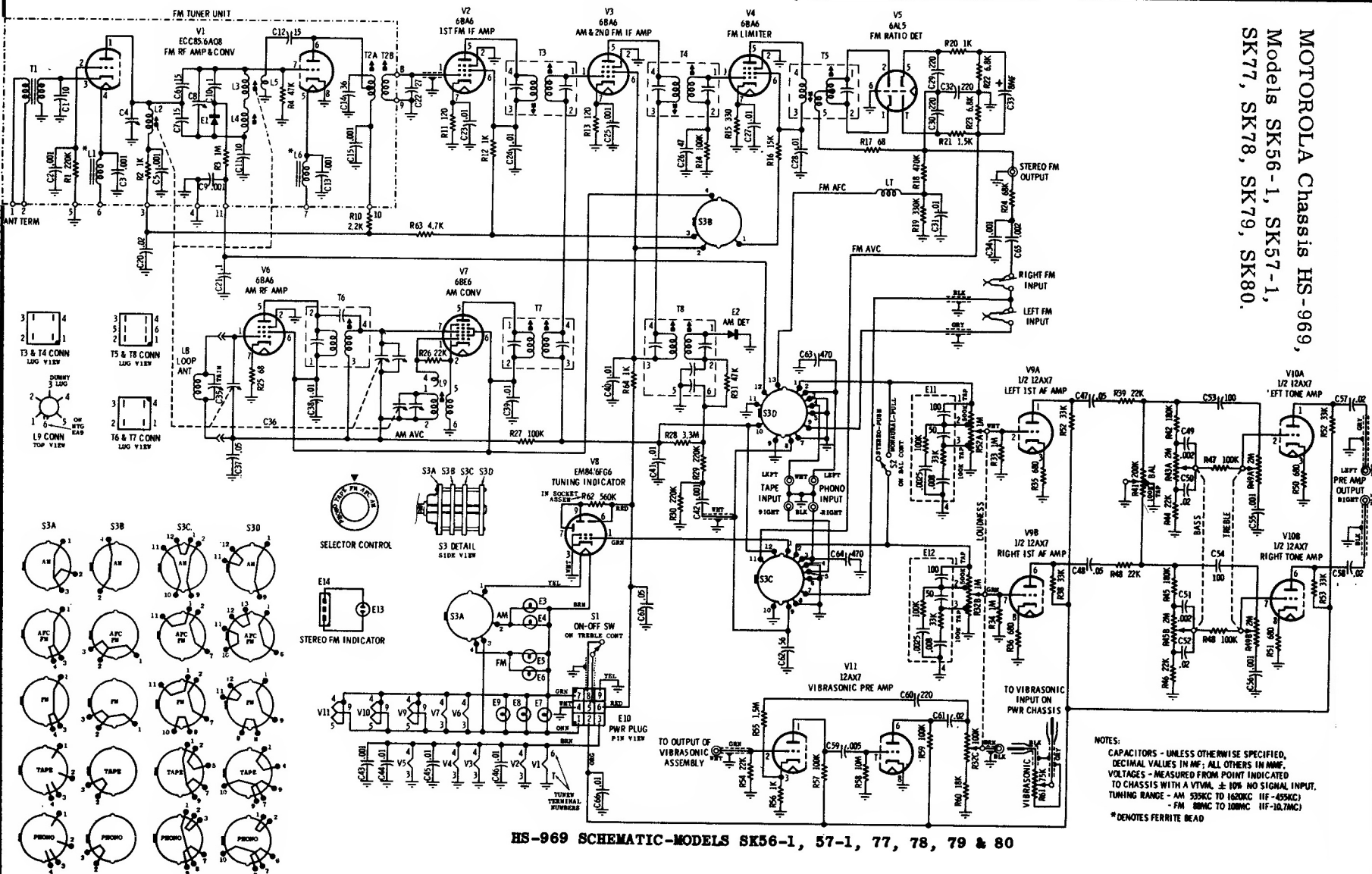
MOTOROLA Chassis HS-969, Models SK56-1, SK57-1, SK77, SK78, SK79, SK80
